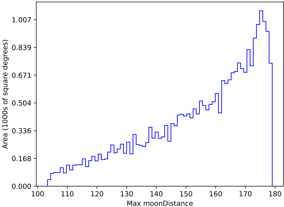
too_ignore_10_4v3.4_10yrs All sky g band: Max moonDistance
