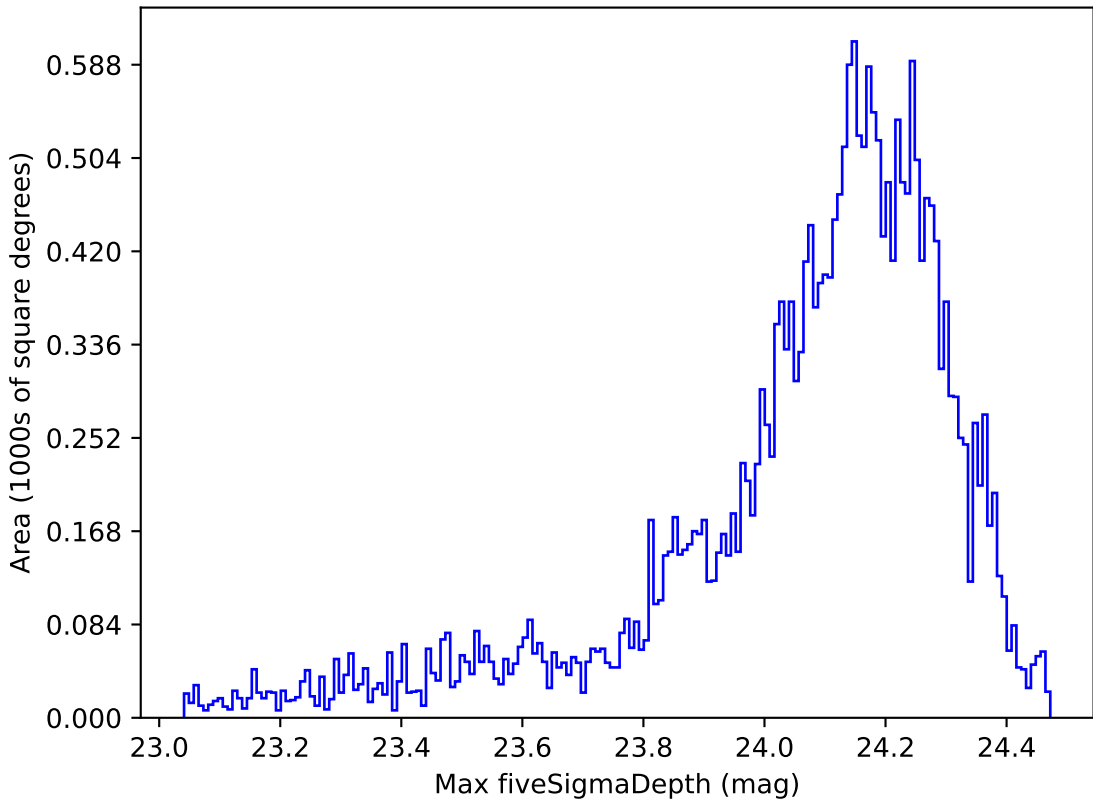
too_ignore_10_4v3.4_10yrs Yr 1 i band: Max fiveSigmaDepth
