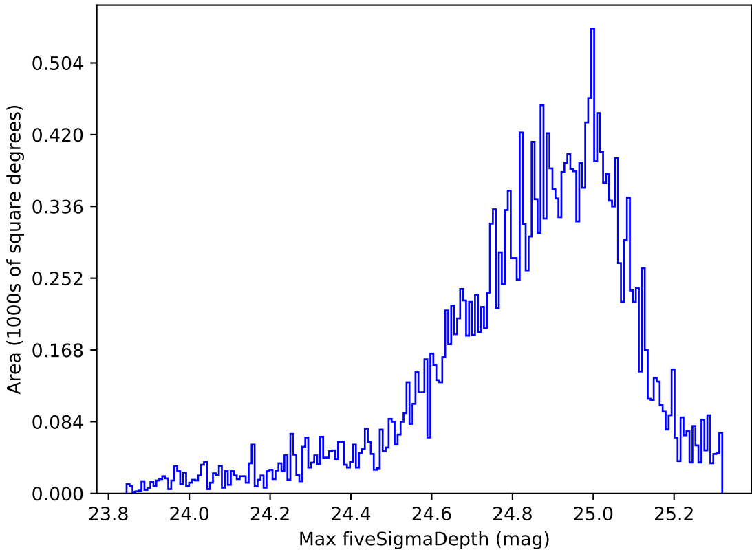
too_ignore_10_4v3.4_10yrs Yr 1 all bands: Max fiveSigmaDepth
