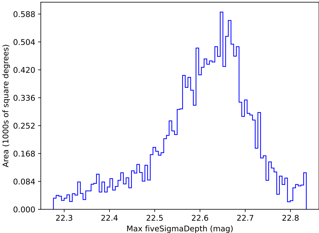
too_ignore_10_4v3.4_10yrs WFD y band: Max fiveSigmaDepth
