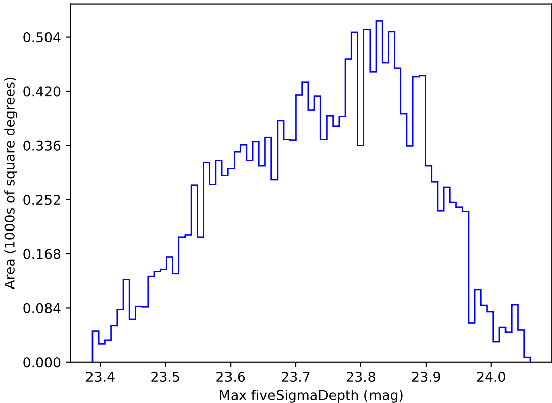
too_ignore_10_4v3.4_10yrs WFD u band: Max fiveSigmaDepth
