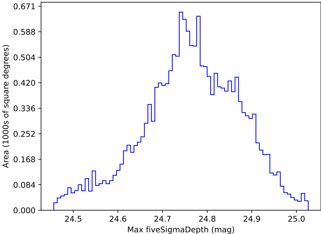
too_ignore_10_4v3.4_10yrs WFD r band: Max fiveSigmaDepth
