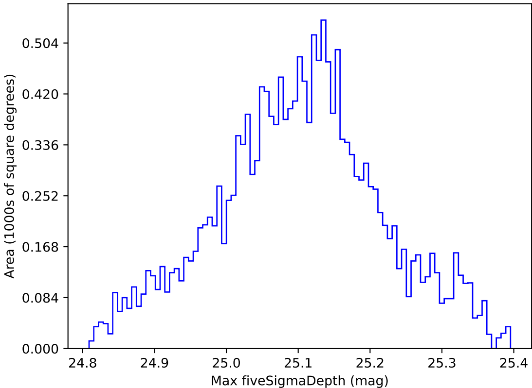
too_ignore_10_4v3.4_10yrs WFD g band: Max fiveSigmaDepth
