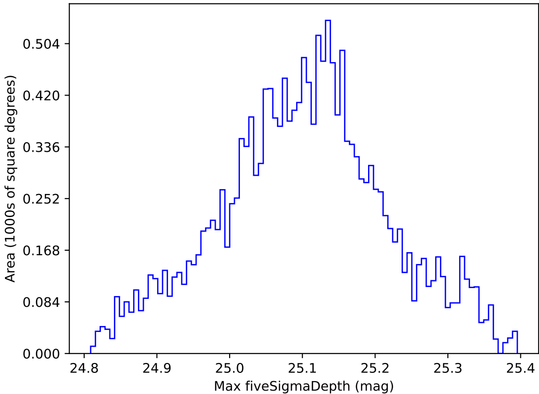
too_ignore_10_4v3.4_10yrs WFD all bands: Max fiveSigmaDepth
