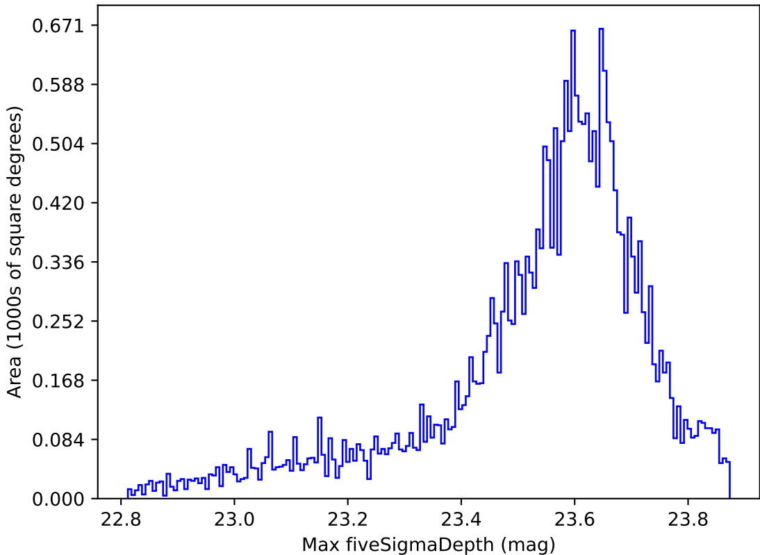
too_ignore_10_4v3.4_10yrs All sky z band: Max fiveSigmaDepth
