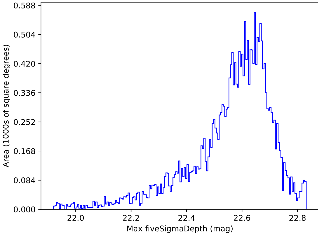
too_ignore_10_4v3.4_10yrs All sky y band: Max fiveSigmaDepth
