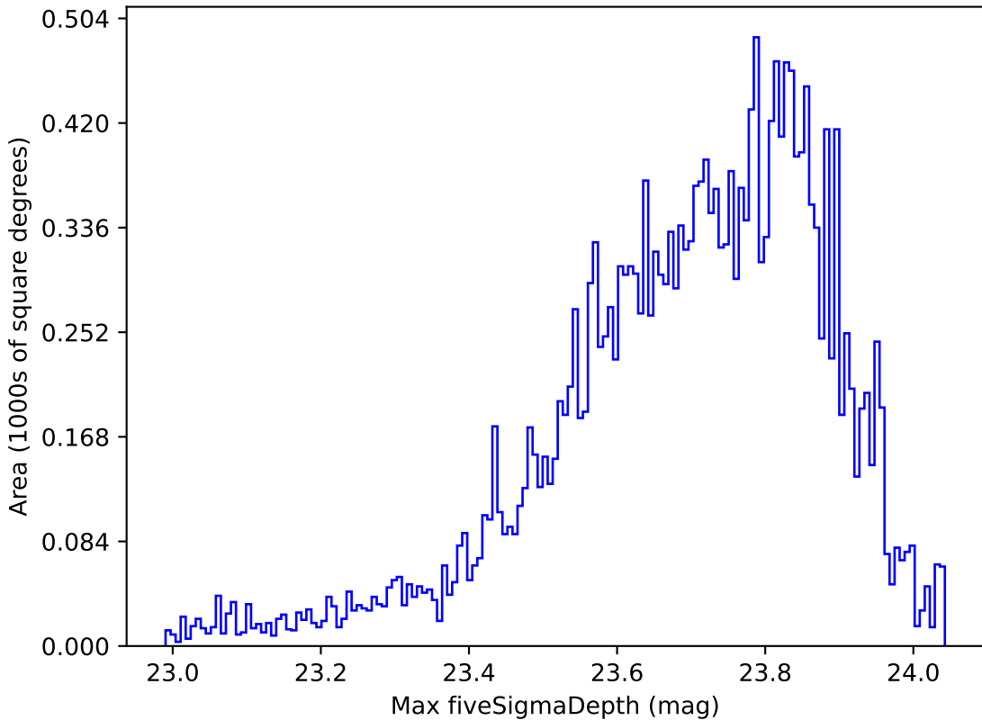
too_ignore_10_4v3.4_10yrs All sky u band: Max fiveSigmaDepth
