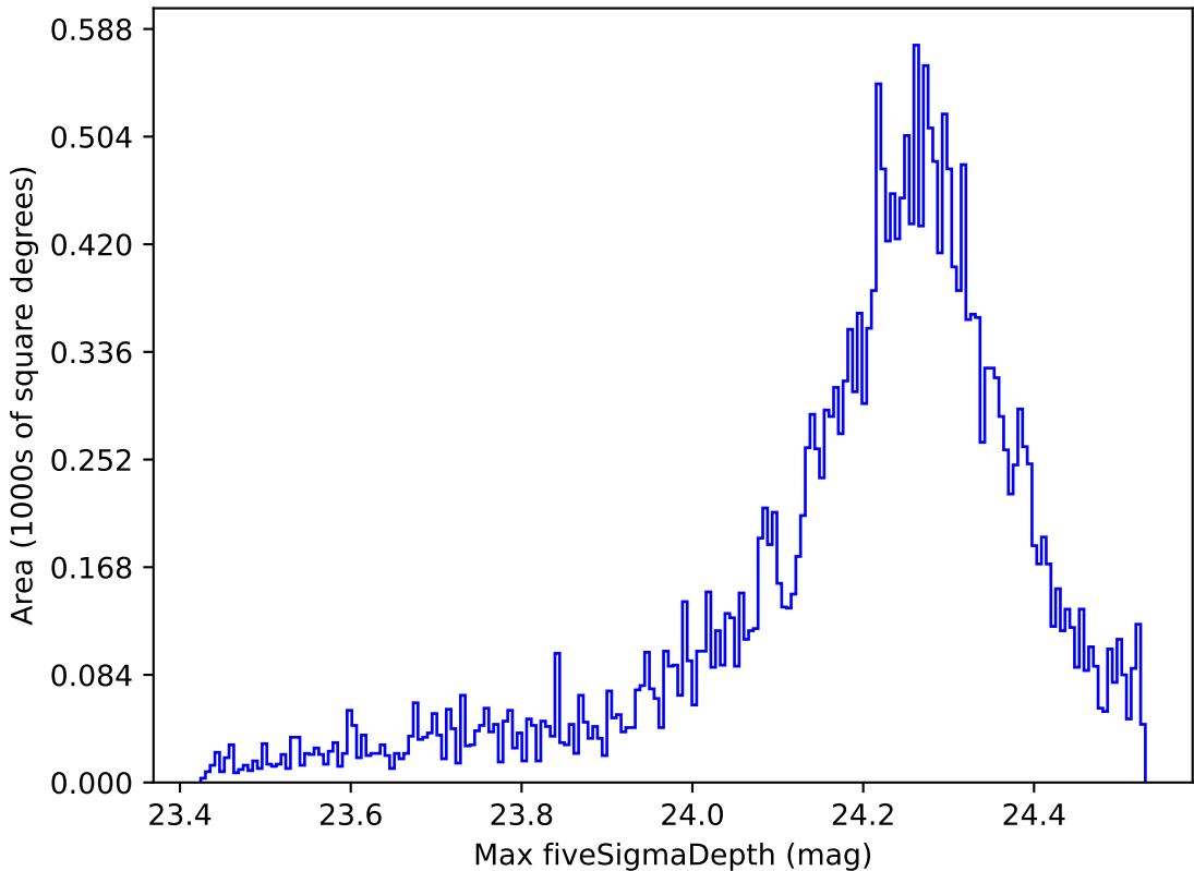
too_ignore_10_4v3.4_10yrs All sky i band: Max fiveSigmaDepth
