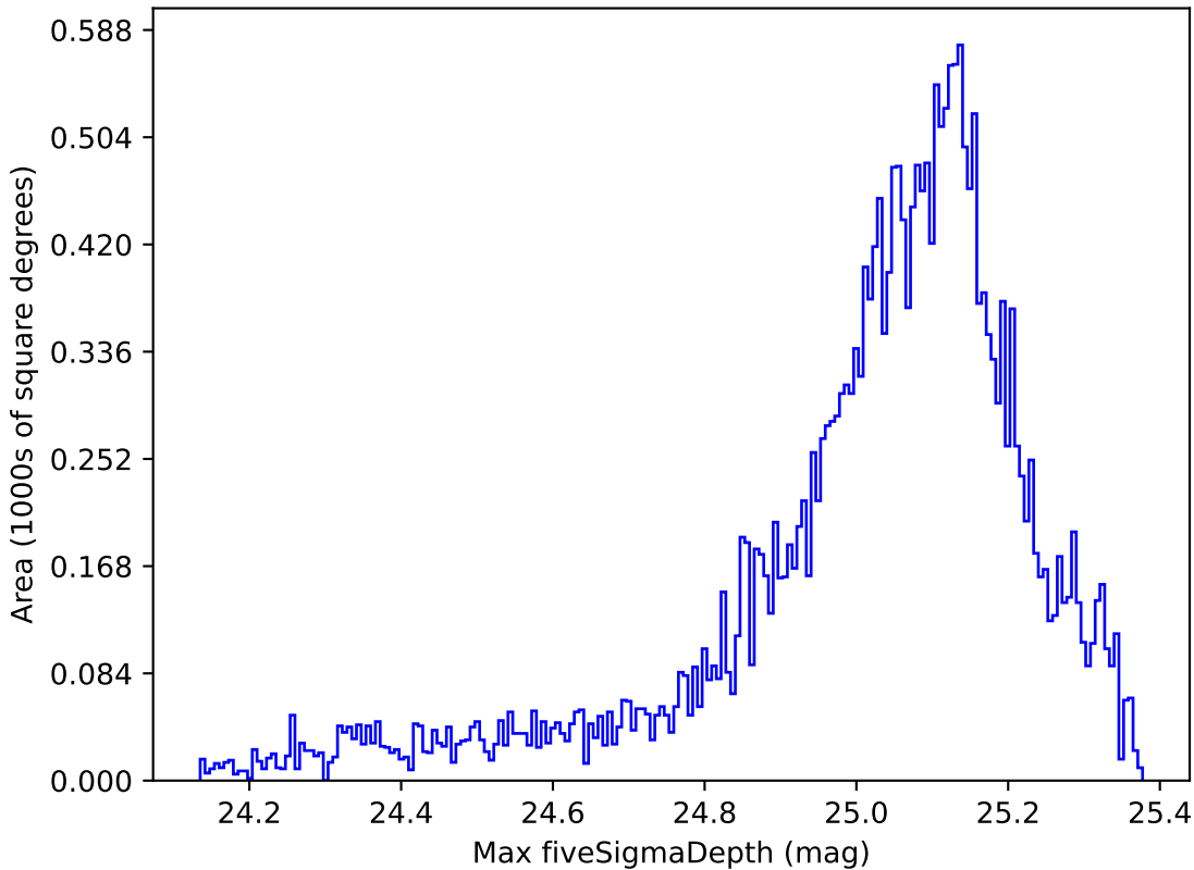
too_ignore_10_4v3.4_10yrs All sky g band: Max fiveSigmaDepth
