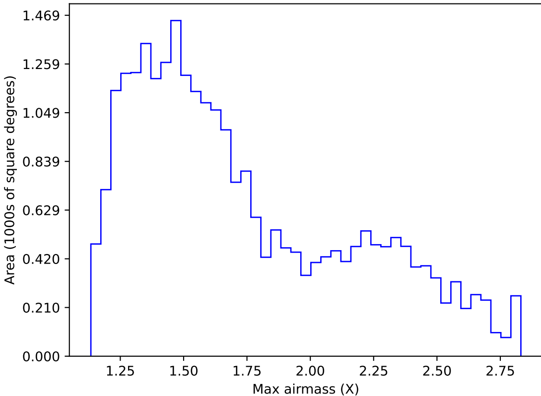
too_ignore_10_4v3.4_10yrs Yr 1 z band: Max airmass
