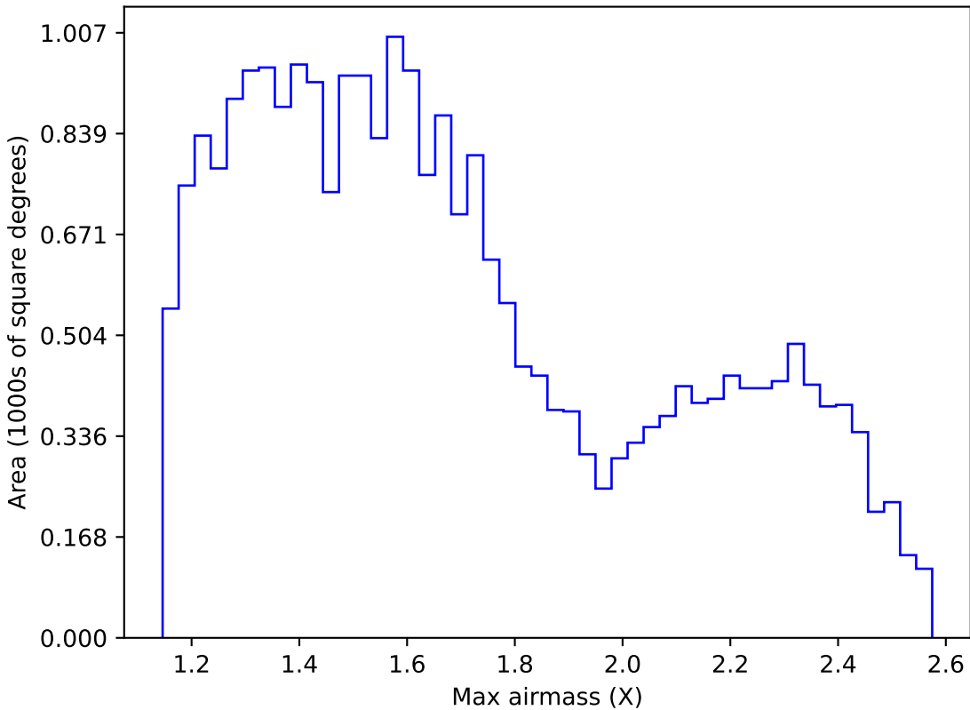
too_ignore_10_4v3.4_10yrs Yr 1 r band: Max airmass
