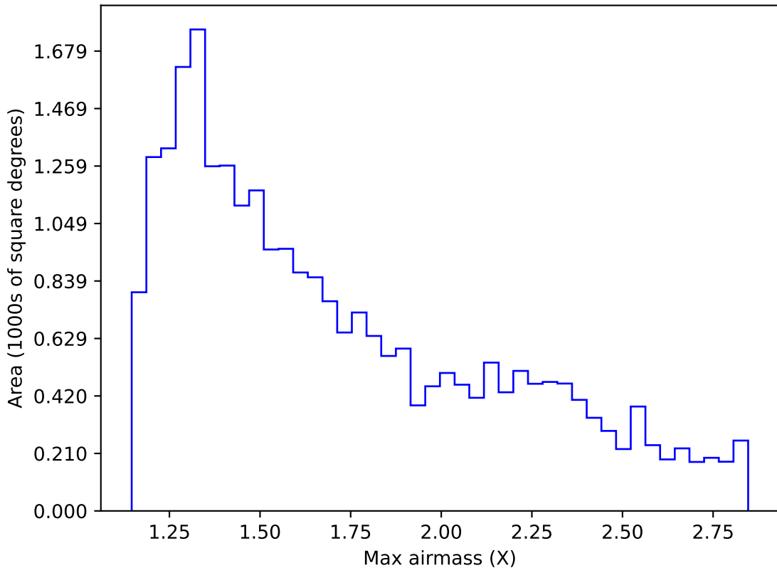
too_ignore_10_4v3.4_10yrs Yr 1 i band: Max airmass
