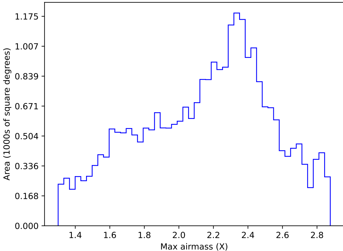
too_ignore_10_4v3.4_10yrs Yr 1 all bands: Max airmass
