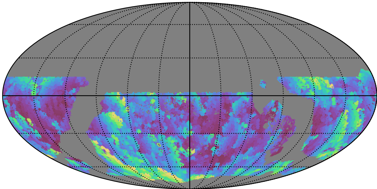
too_ignore_10_4v3.4_10yrs WFD u band: Max airmass
