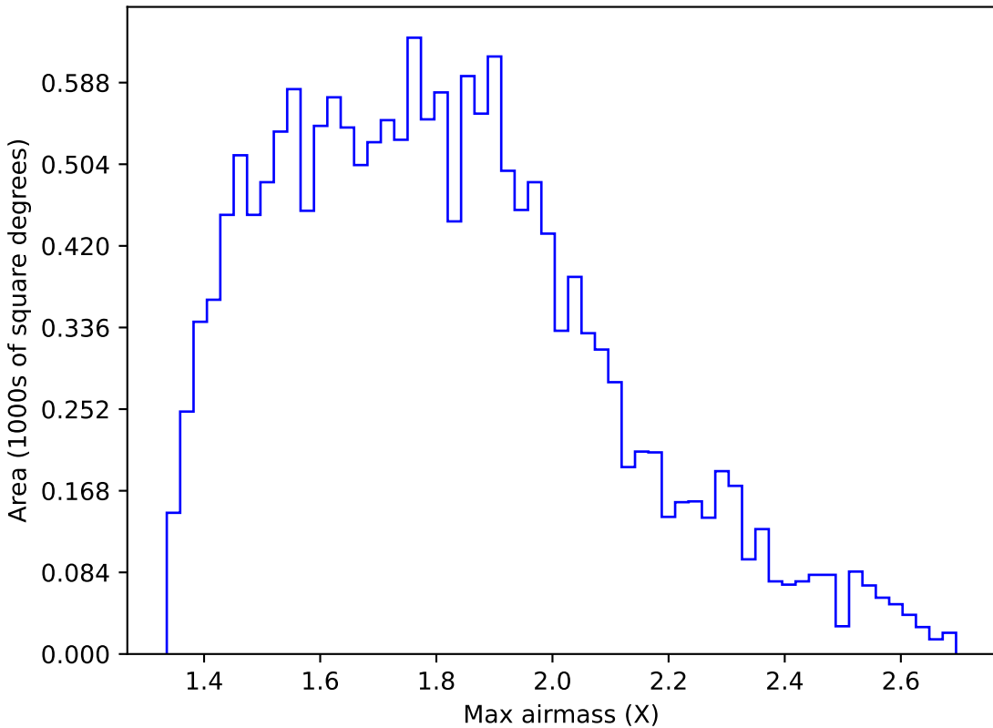
too_ignore_10_4v3.4_10yrs WFD u band: Max airmass
