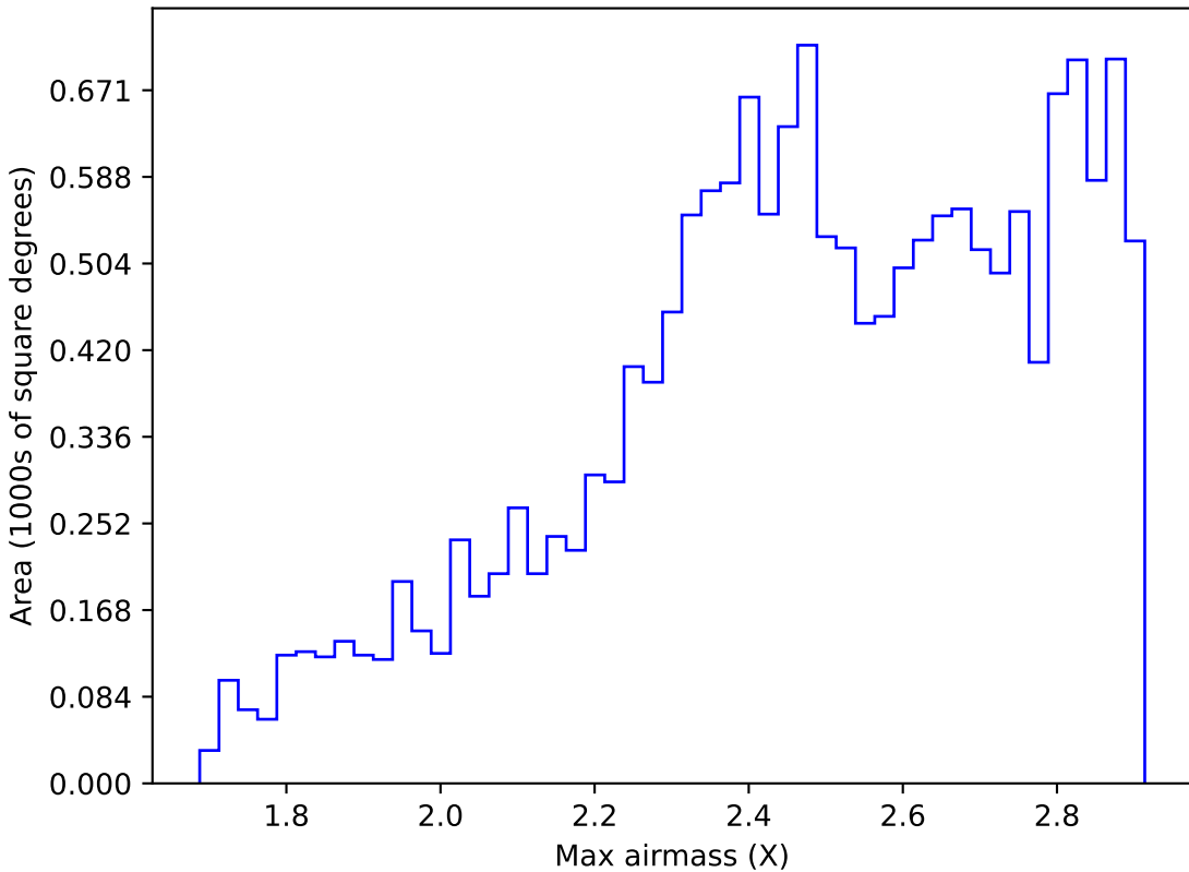
too_ignore_10_4v3.4_10yrs WFD i band: Max airmass
