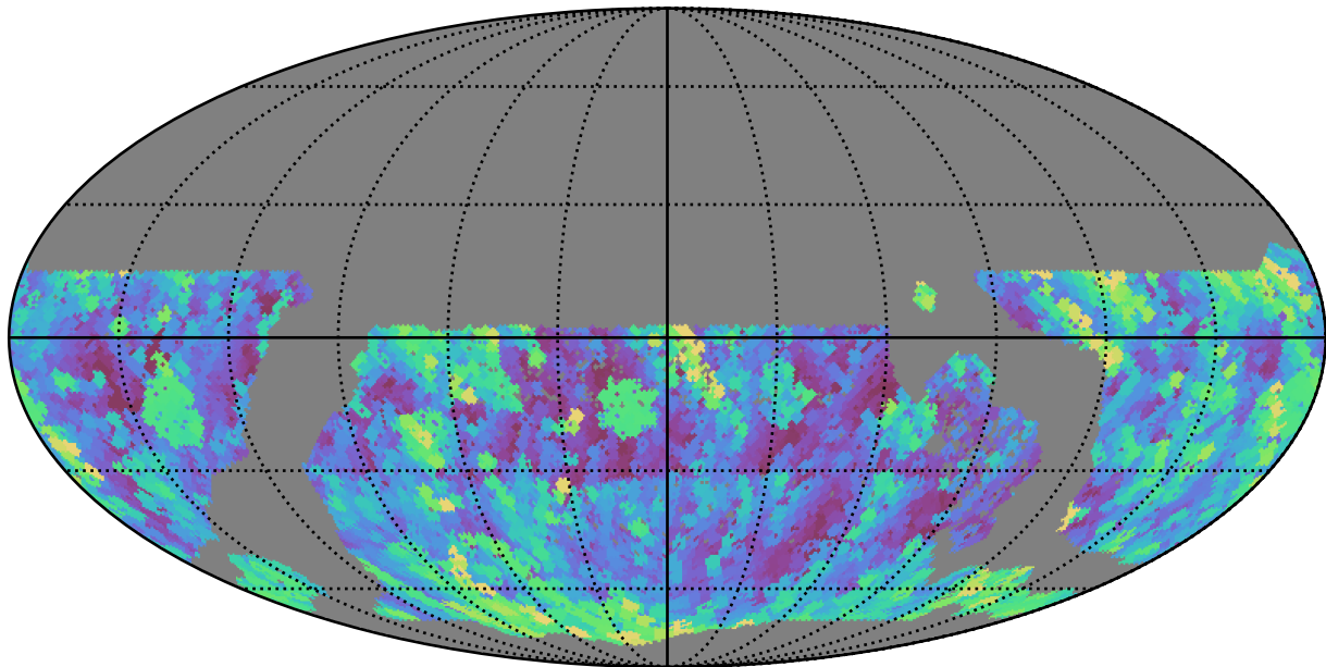
too_ignore_10_4v3.4_10yrs WFD g band: Max airmass
