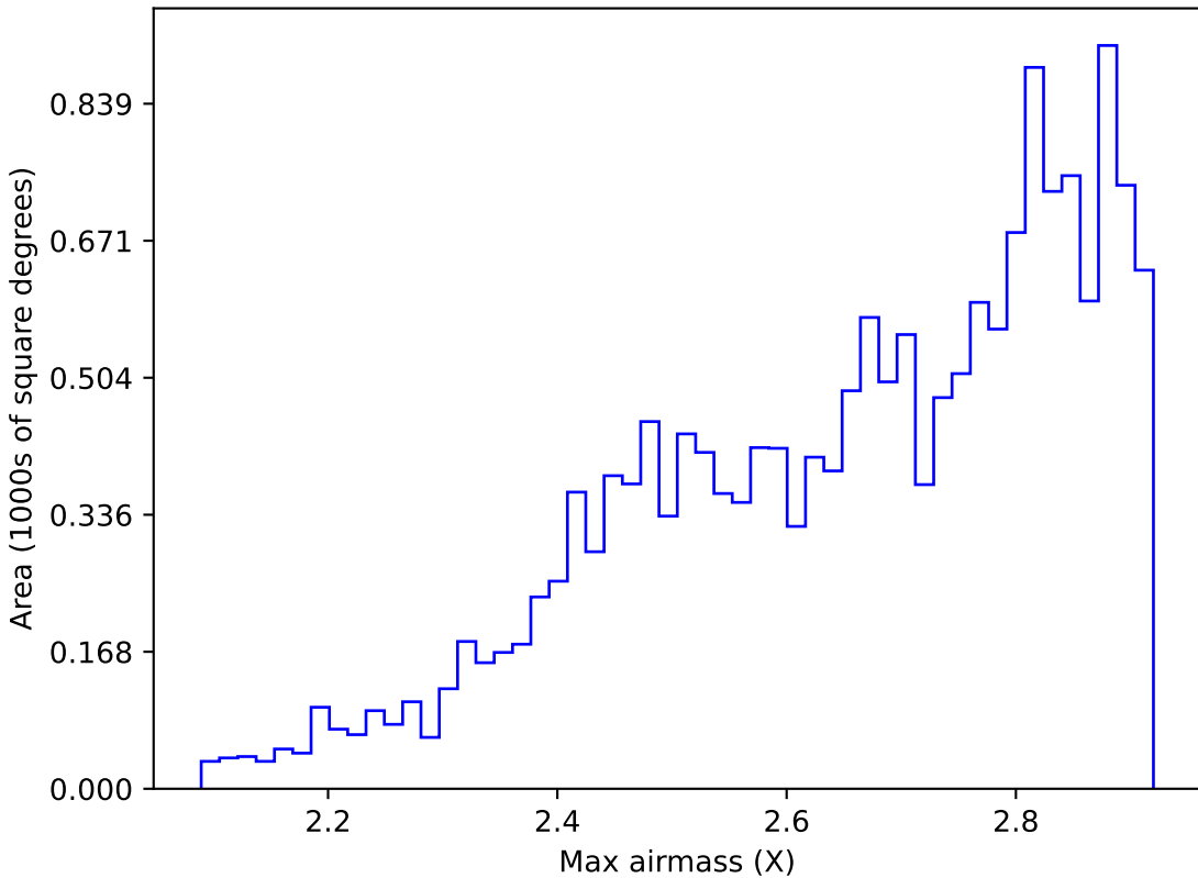
too_ignore_10_4v3.4_10yrs WFD all bands: Max airmass
