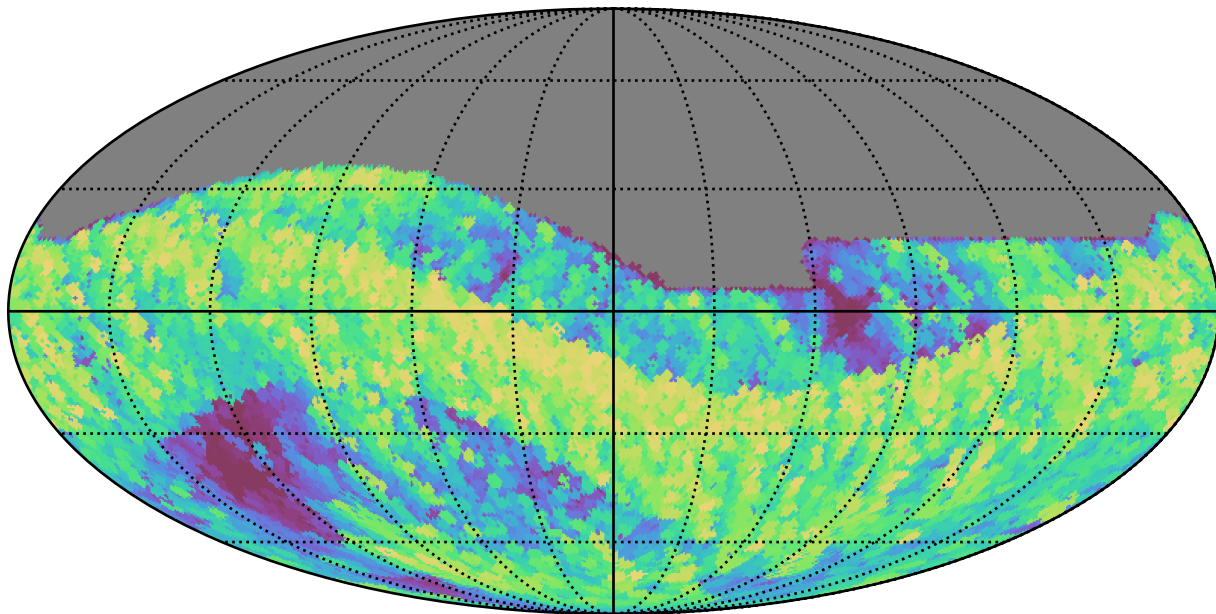
too_ignore_10_4v3.4_10yrs All sky z band: Max airmass
