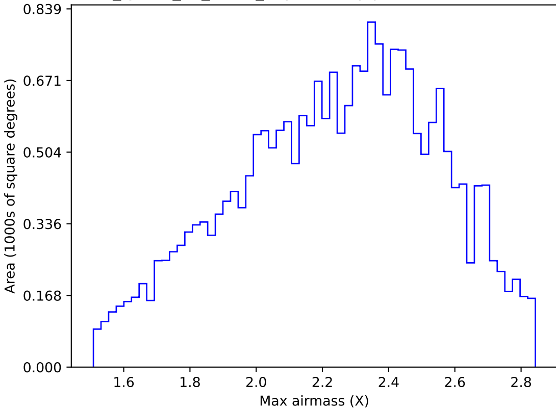
too_ignore_10_4v3.4_10yrs All sky y band: Max airmass
