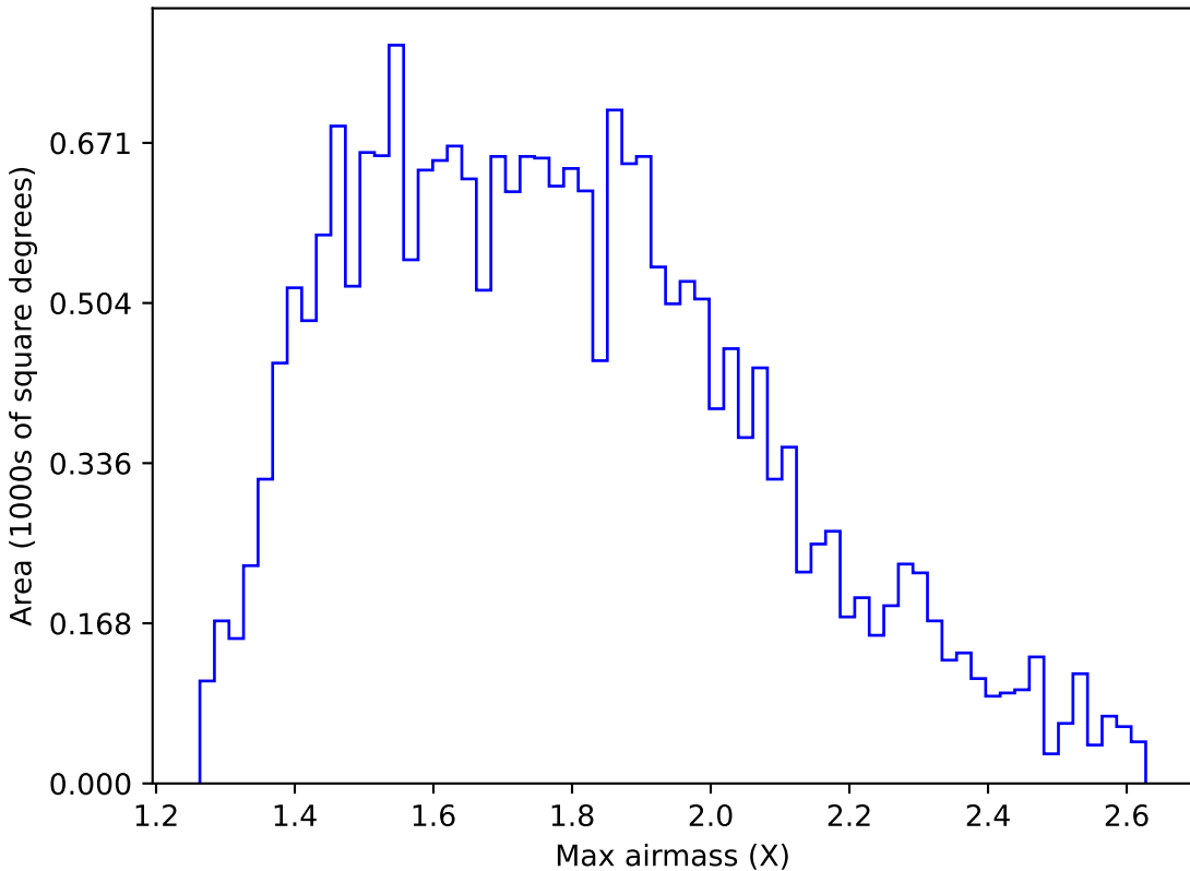
too_ignore_10_4v3.4_10yrs All sky u band: Max airmass
