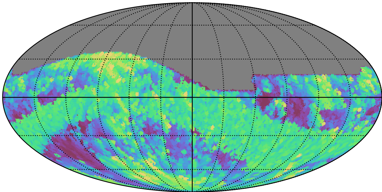
too_ignore_10_4v3.4_10yrs All sky r band: Max airmass
