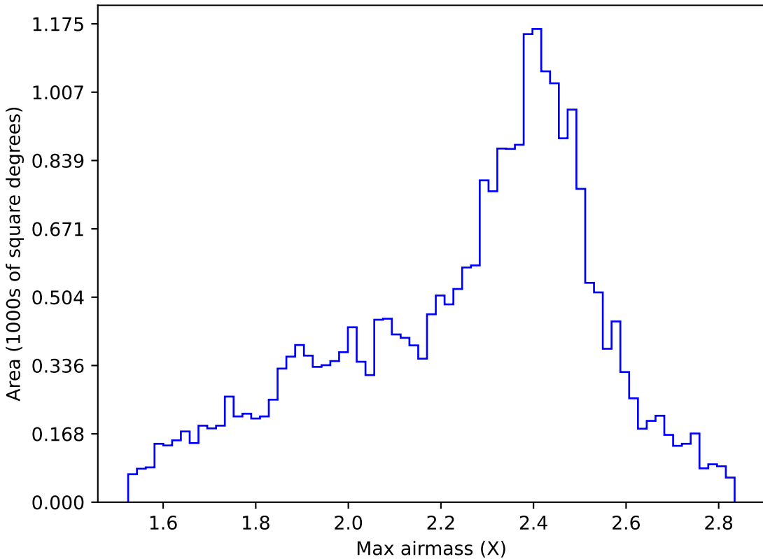
too_ignore_10_4v3.4_10yrs All sky r band: Max airmass
