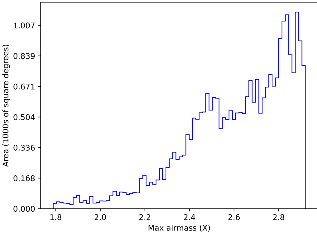
too_ignore_10_4v3.4_10yrs All sky all bands: Max airmass
