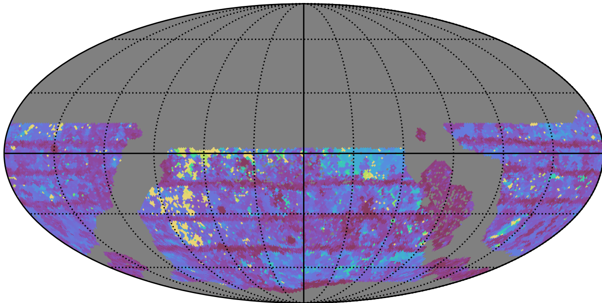
too_ignore_10_4v3.4_10yrs WFD z band: Max Inter-Night Gap
