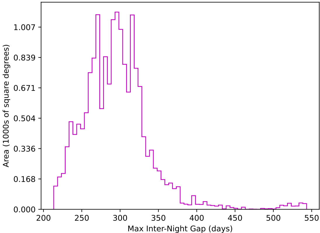
too_ignore_10_4v3.4_10yrs WFD z band: Max Inter-Night Gap
