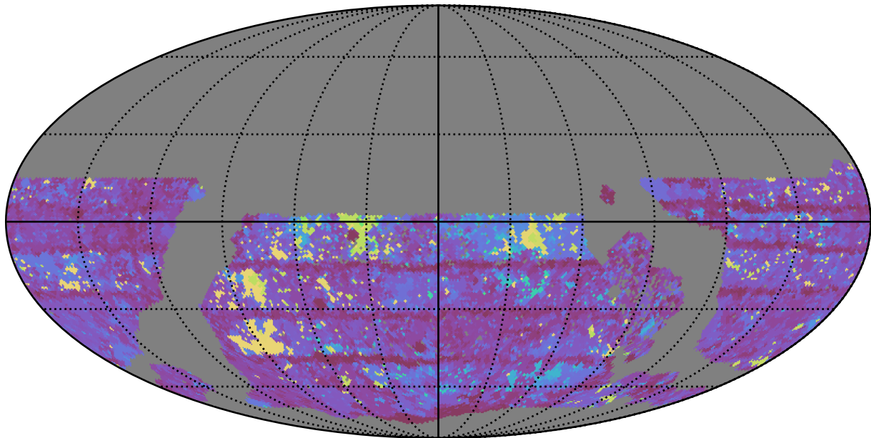
too_ignore_10_4v3.4_10yrs WFD y band: Max Inter-Night Gap
