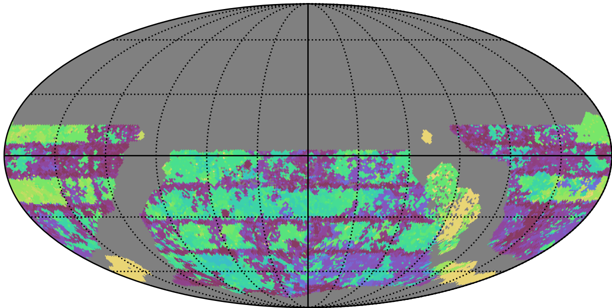
too_ignore_10_4v3.4_10yrs WFD u band: Max Inter-Night Gap
