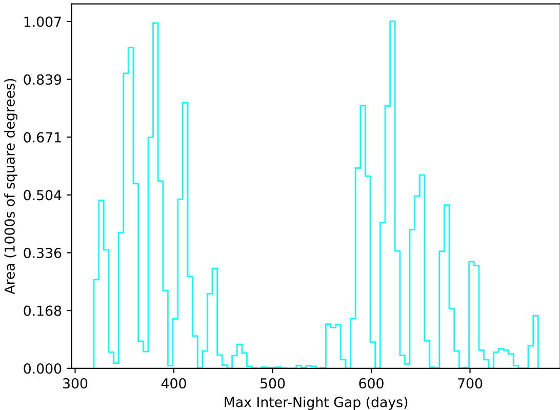
too_ignore_10_4v3.4_10yrs WFD u band: Max Inter-Night Gap
