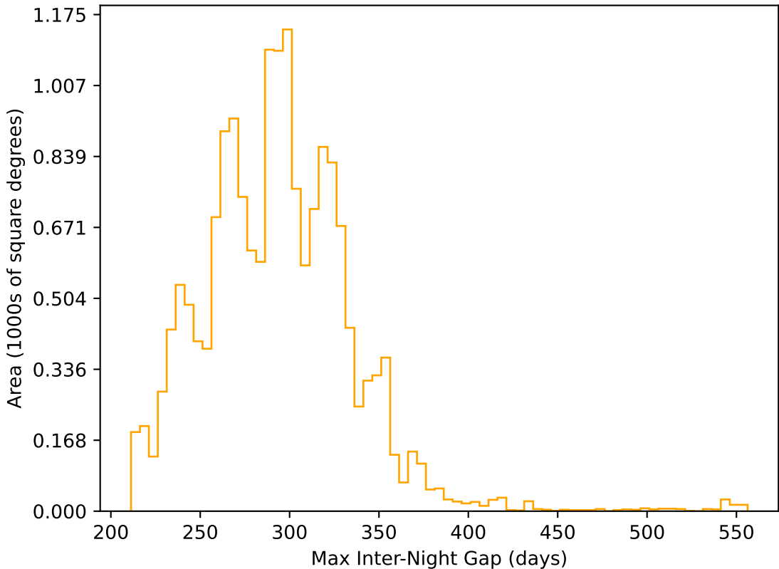
too_ignore_10_4v3.4_10yrs WFD r band: Max Inter-Night Gap
