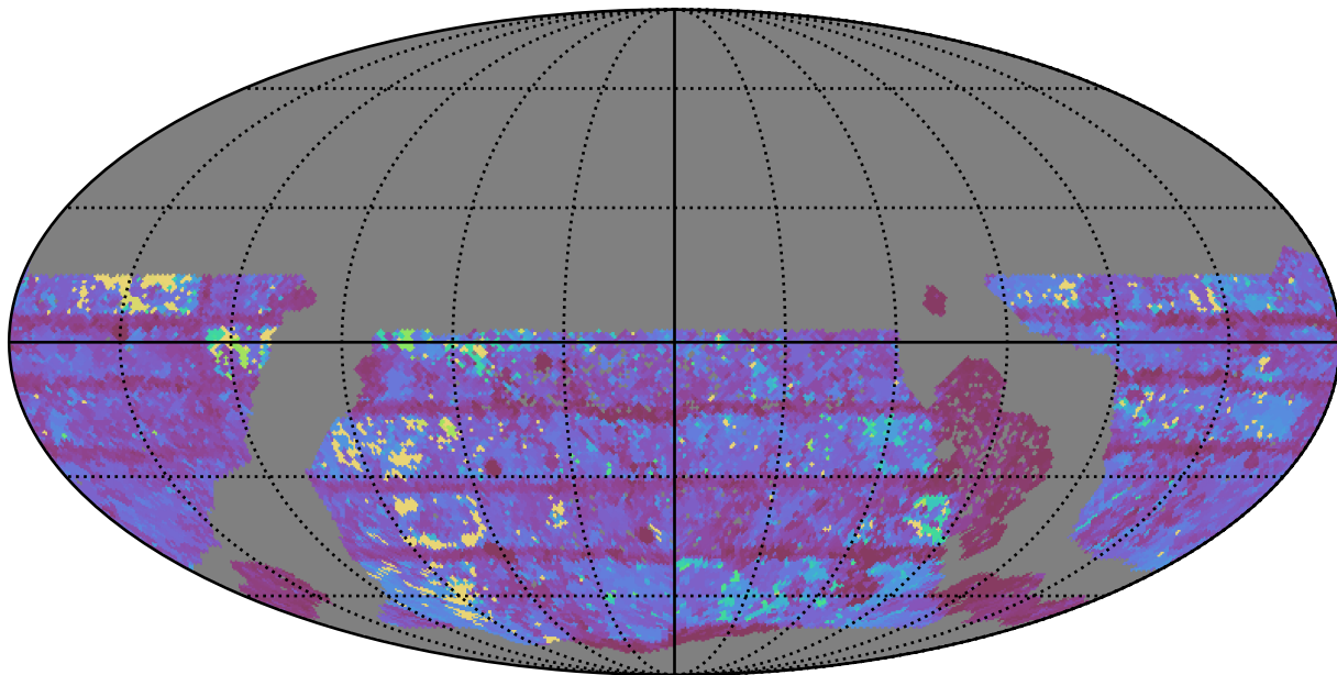
too_ignore_10_4v3.4_10yrs WFD i band: Max Inter-Night Gap
