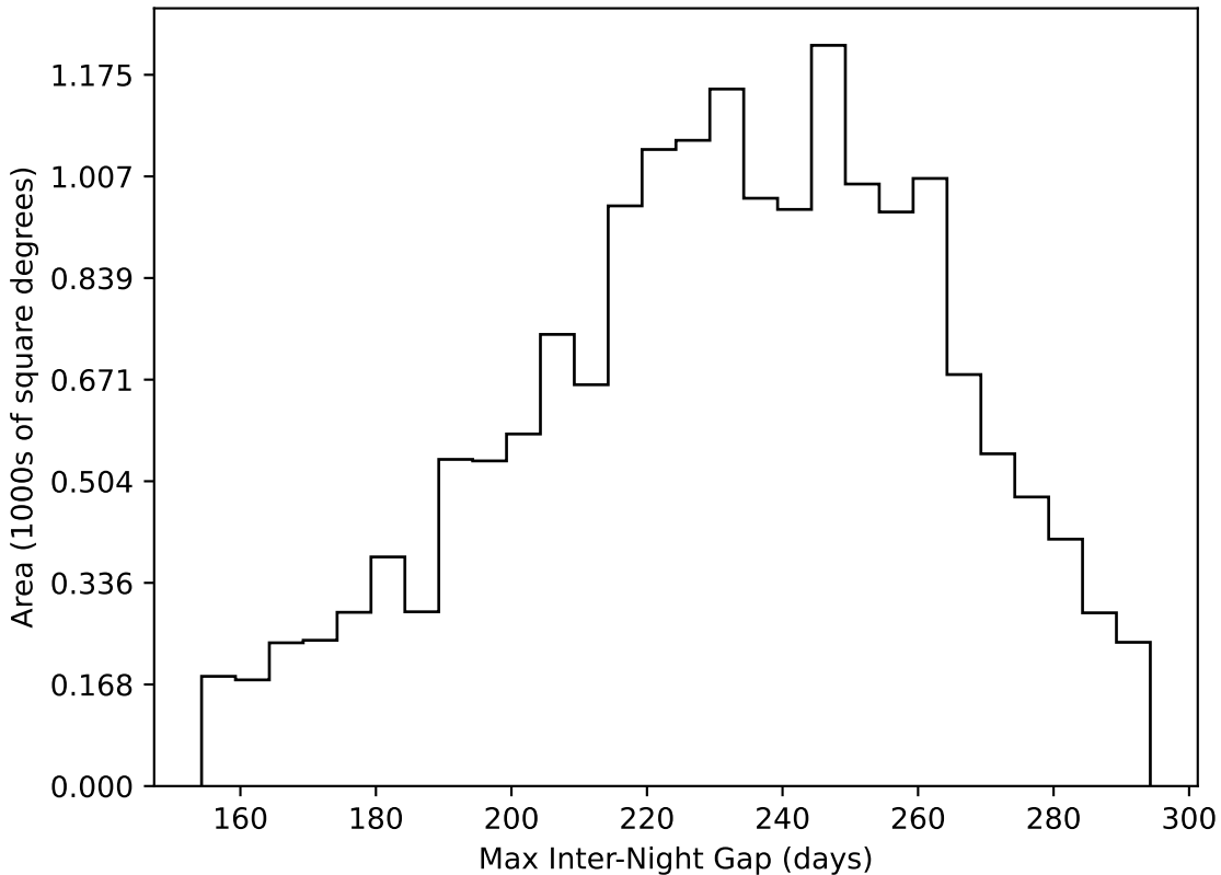
too_ignore_10_4v3.4_10yrs WFD all bands: Max Inter-Night Gap
