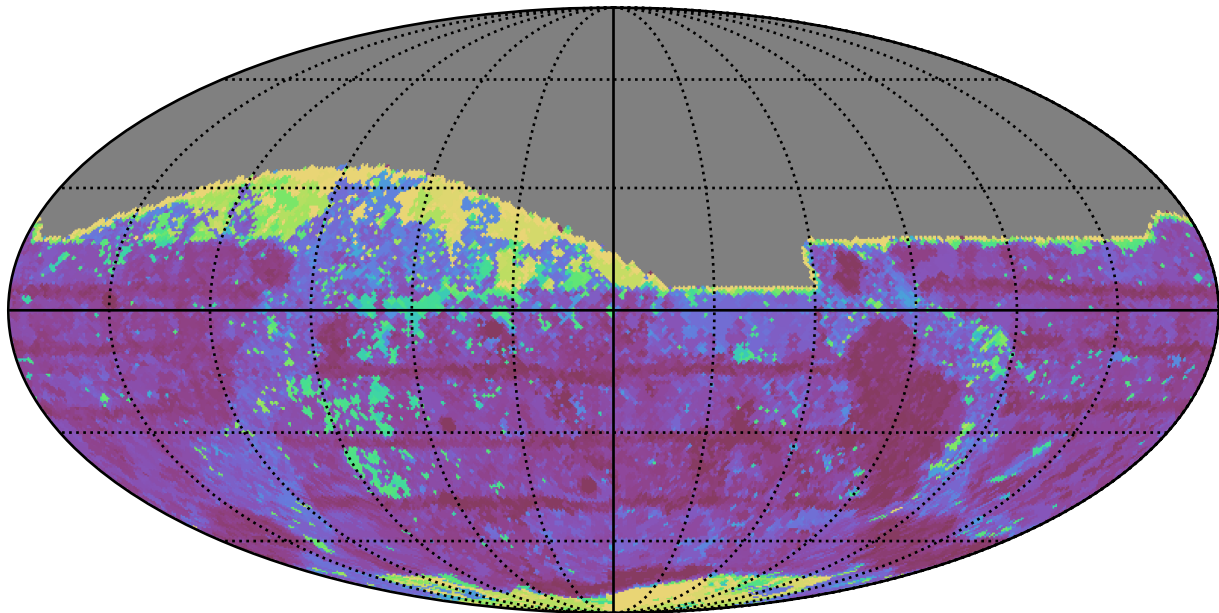
too_ignore_10_4v3.4_10yrs All sky z band: Max Inter-Night Gap
