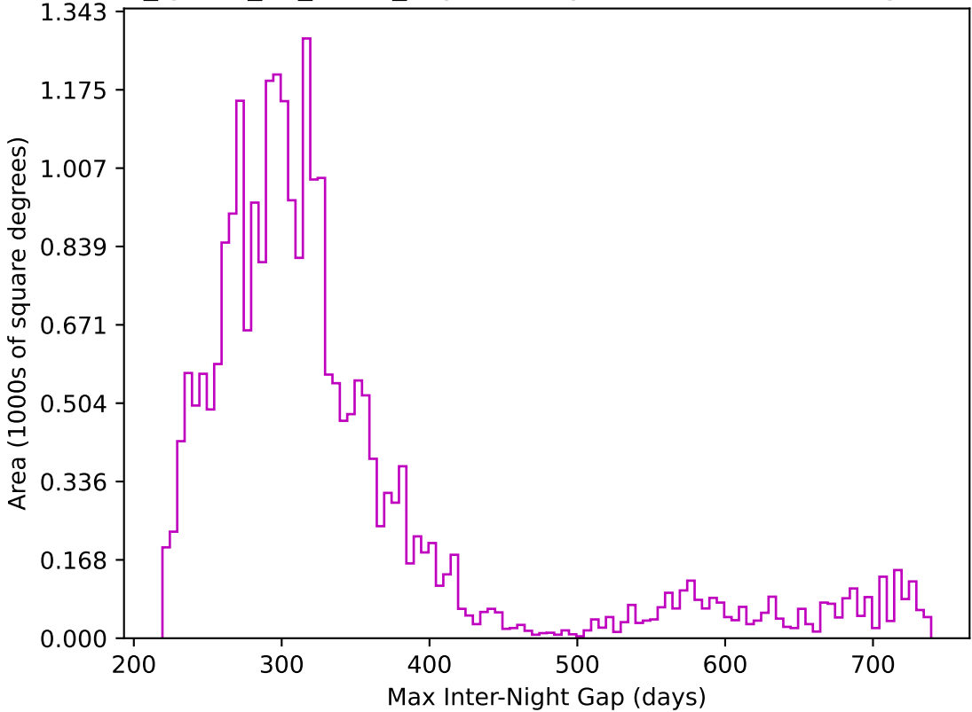
too_ignore_10_4v3.4_10yrs All sky z band: Max Inter-Night Gap
