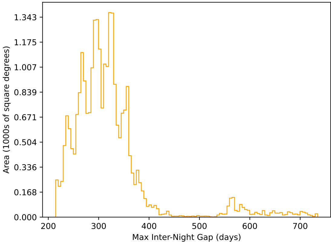
too_ignore_10_4v3.4_10yrs All sky r band: Max Inter-Night Gap
