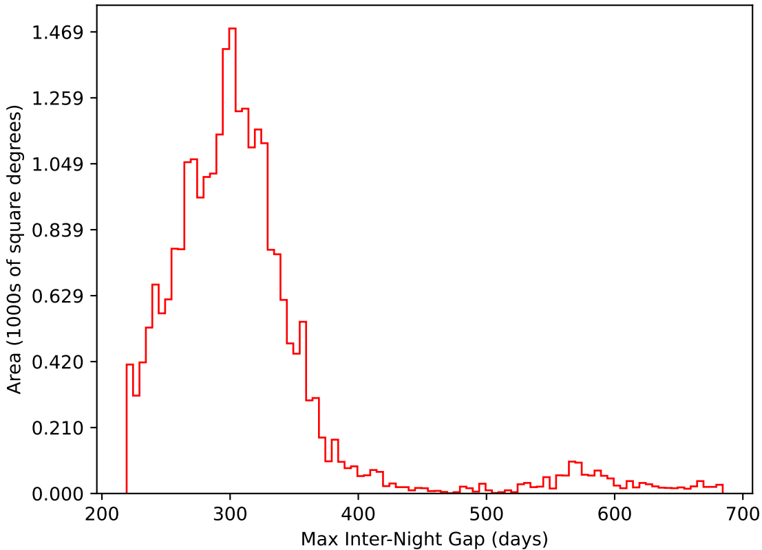
too_ignore_10_4v3.4_10yrs All sky i band: Max Inter-Night Gap
