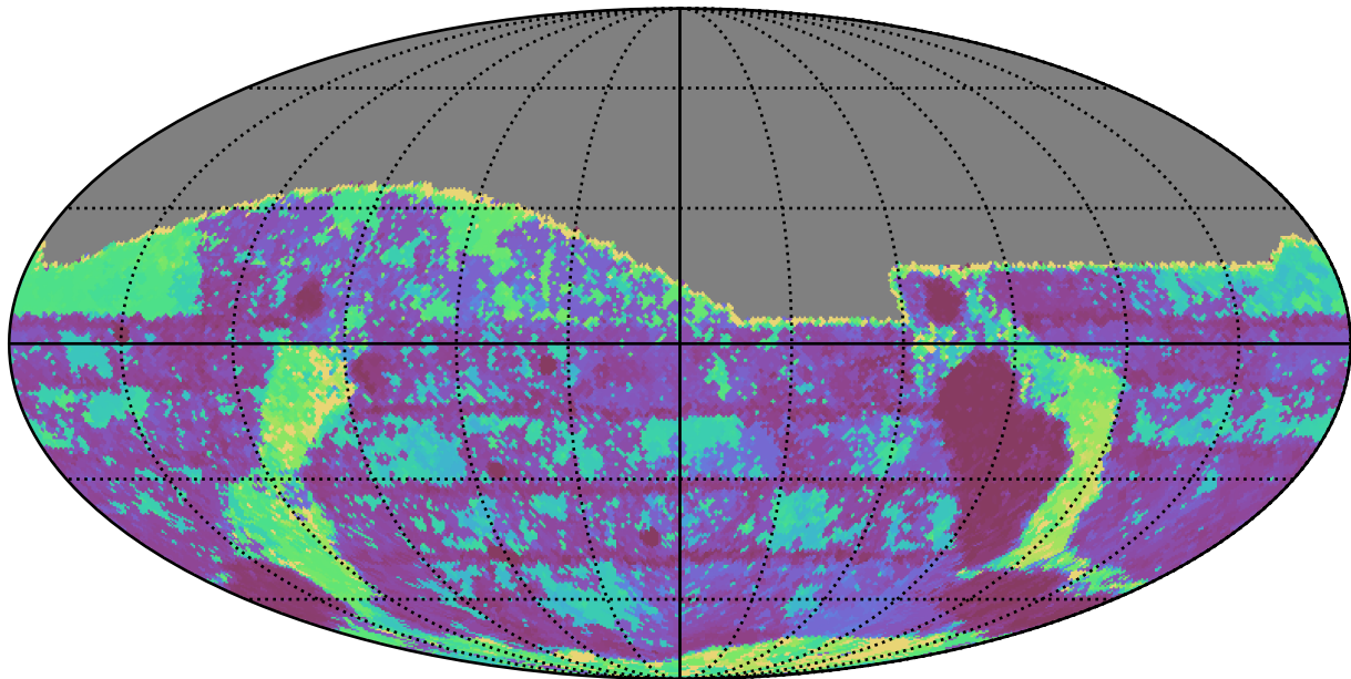
too_ignore_10_4v3.4_10yrs All sky g band: Max Inter-Night Gap
