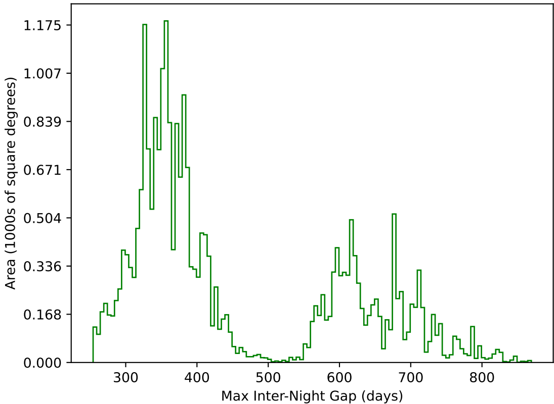
too_ignore_10_4v3.4_10yrs All sky g band: Max Inter-Night Gap
