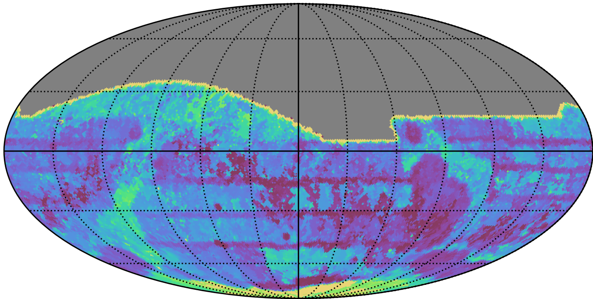
too_ignore_10_4v3.4_10yrs All sky all bands: Max Inter-Night Gap
