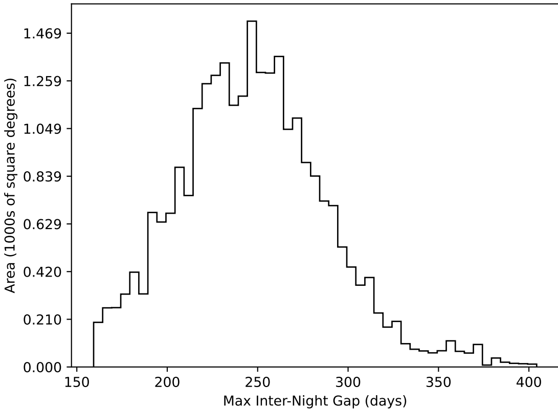
too_ignore_10_4v3.4_10yrs All sky all bands: Max Inter-Night Gap
