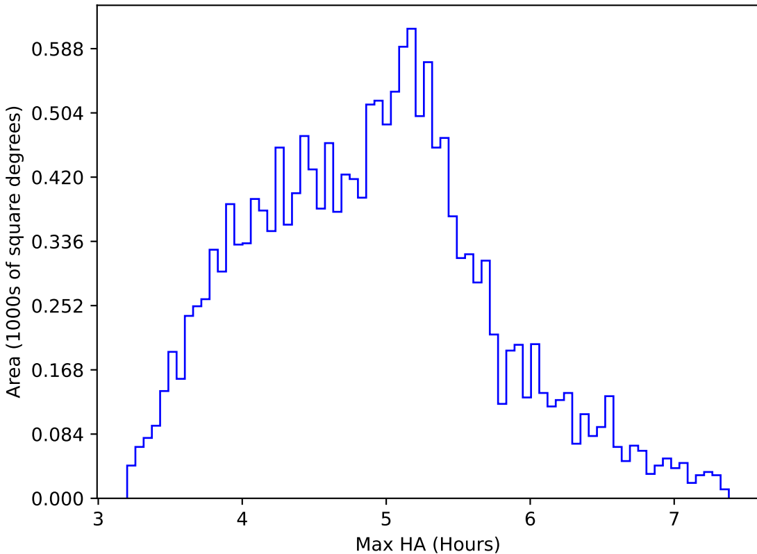
too_ignore_10_4v3.4_10yrs WFD z band: Max HA
