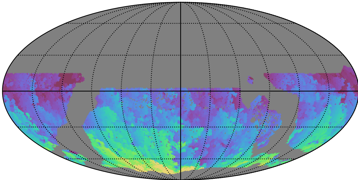
too_ignore_10_4v3.4_10yrs WFD u band: Max HA
