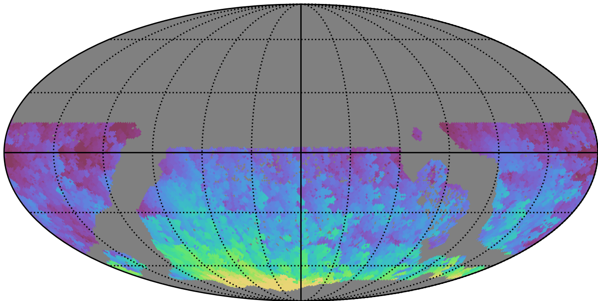
too_ignore_10_4v3.4_10yrs WFD r band: Max HA
