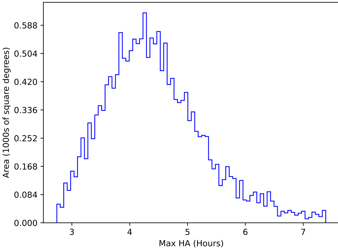
too_ignore_10_4v3.4_10yrs WFD r band: Max HA
