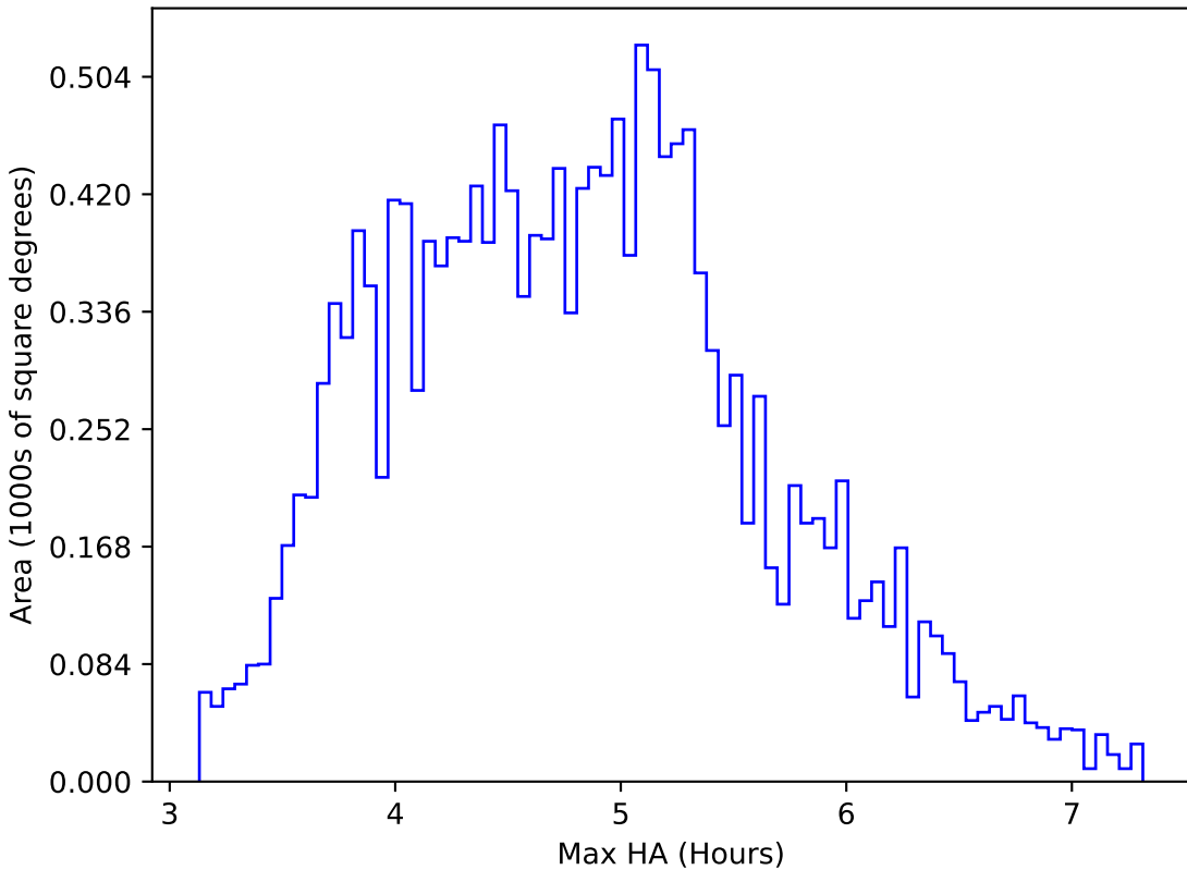
too_ignore_10_4v3.4_10yrs WFD i band: Max HA
