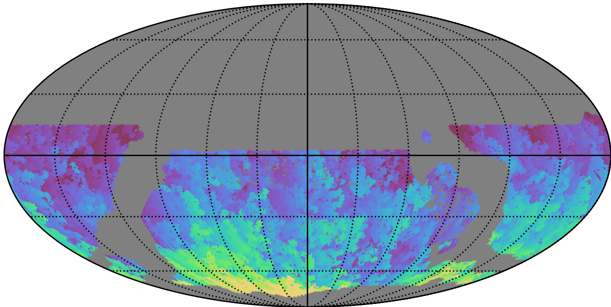
too_ignore_10_4v3.4_10yrs WFD g band: Max HA
